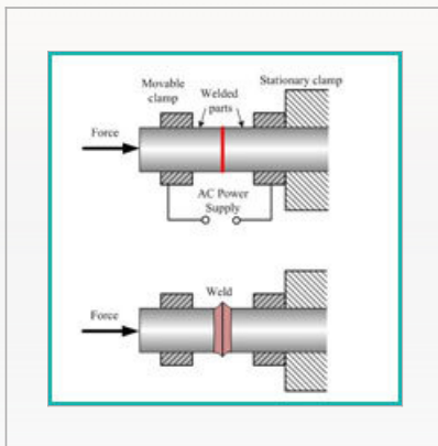
Butt Welding
